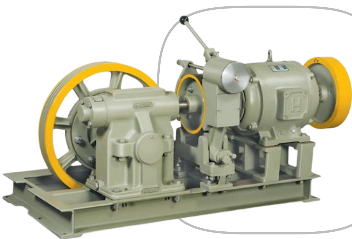
TRACTION MACHINE
